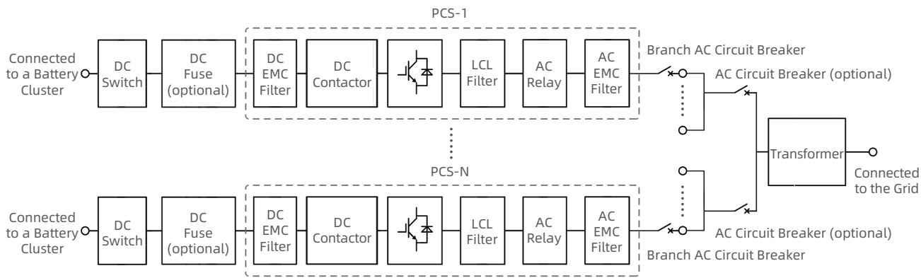
N≤24: Double-winding Transformer
