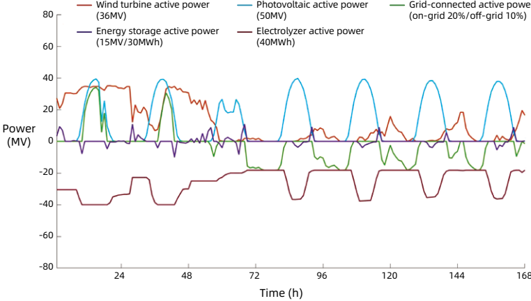
Active power dispatching curve of grid-connected power plant
