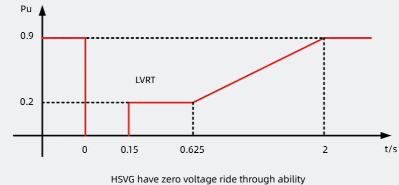
HSVG have zero voltage ride through ability
