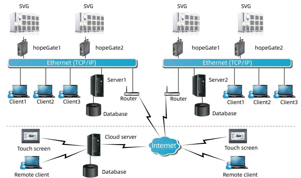
(hopeView monitoring system network diagram)
