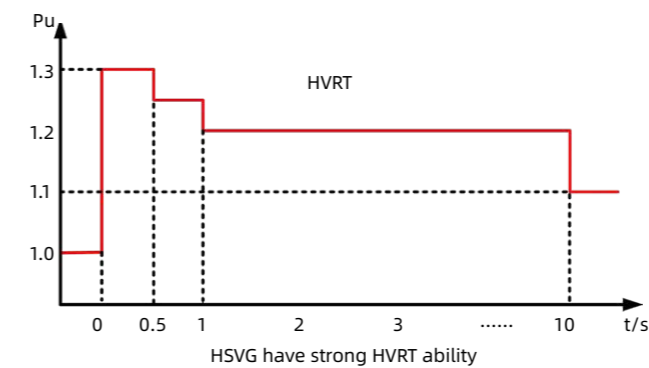
HSVG have strong HVRT ability
