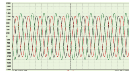
(Before compensation - grid voltage imbalance is serious)
