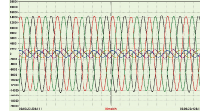
(After compensation - grid voltage imbalance is small)
